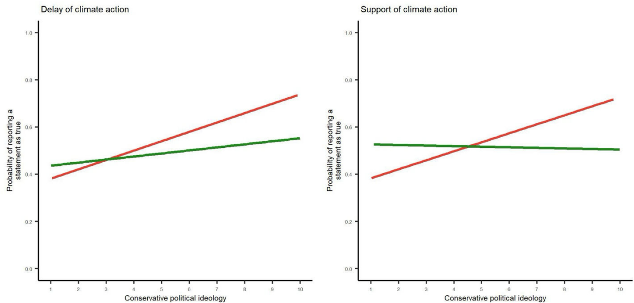
Figure B4. Mean probability of each statement of the truth discernment task to be reported as true according to the bias of the right hypothesis. Simulated data.
